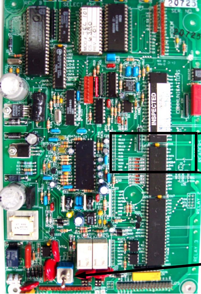
MAIN BOARD
