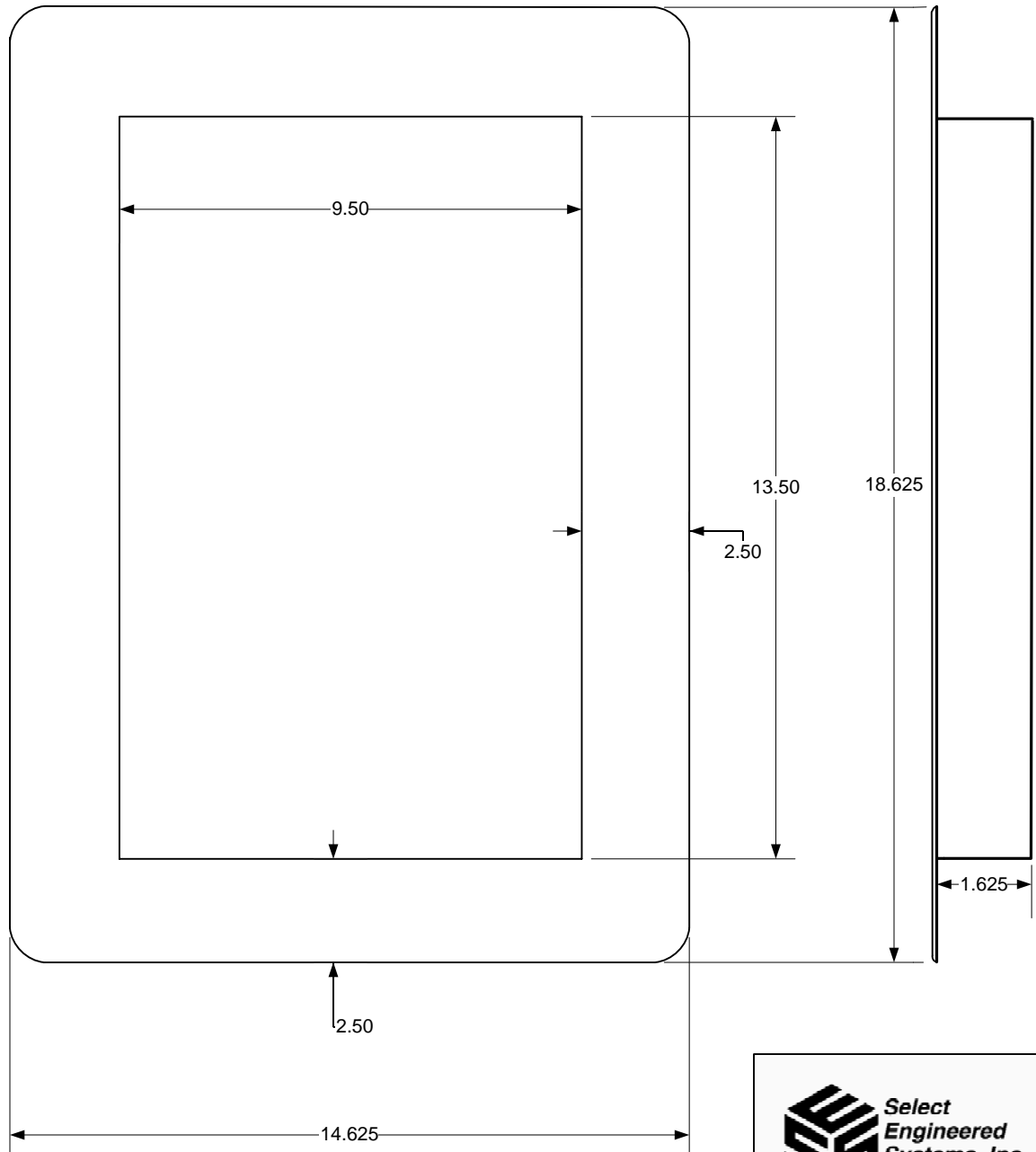
FRONT VIEW
